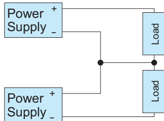
Fig.4.1 Series Operation
