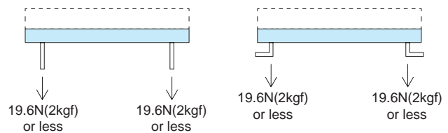
Fig.6.6 Strength of Input/Output Pin Terminals for SU/SUC
