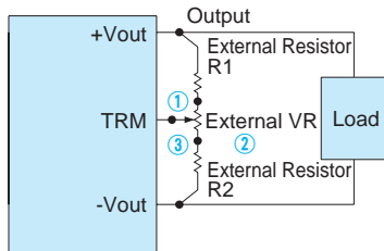
Fig.2.2 Connecting External Devices
